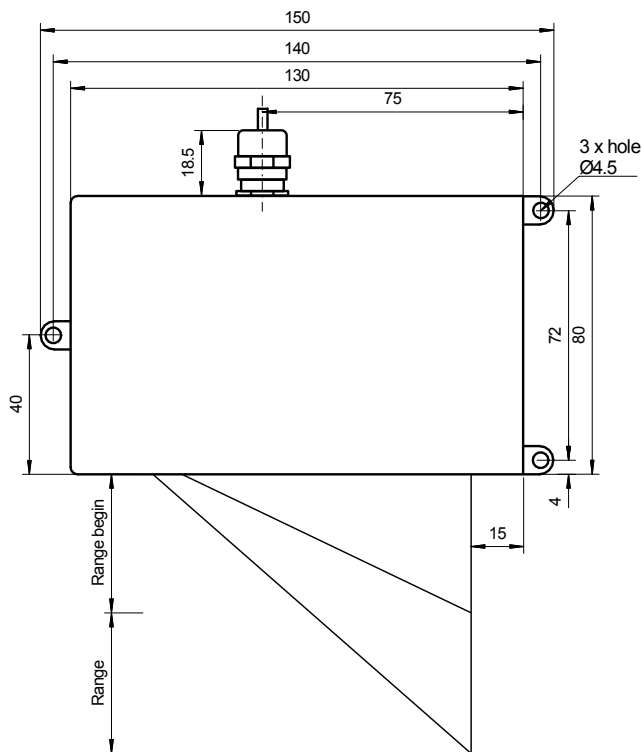
M9-i-40/500/750 weight 600 g, cable length 0.25 m
