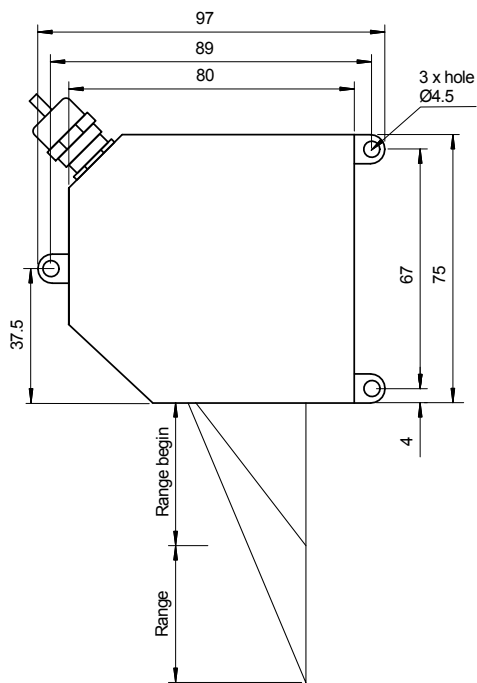
M9-i-2/10/20/50/100/200/250VT weight 550 g, cable length 0.25 m
