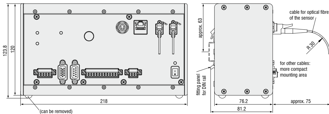
Controller IFC2471
